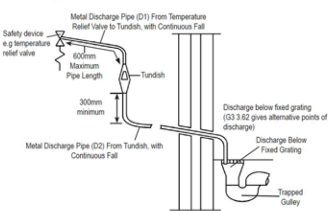
Discharge pipe arrangement
