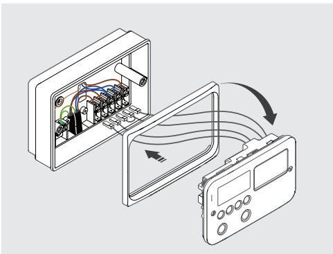
Adaptor plate for retrofitting
