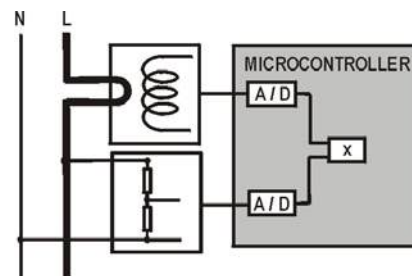
Fig. 10: Metering element
