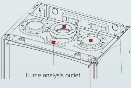
Air intake manifold for split exhaust systems
